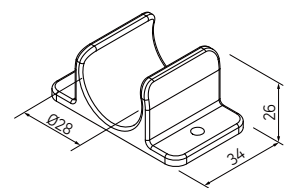
PLASTIC HINGE
