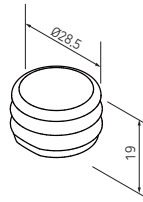
PIPE INNER CAP
