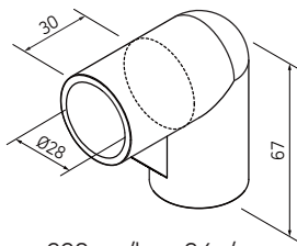
PLASTIC JOINT L TYPE
