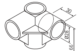
PLASTIC JOINT 3 WAY TYPE
