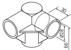
PJ-104C (IV) PLASTIC JOINT TOP FLAT TYPE
