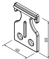
BAND-HOOK
